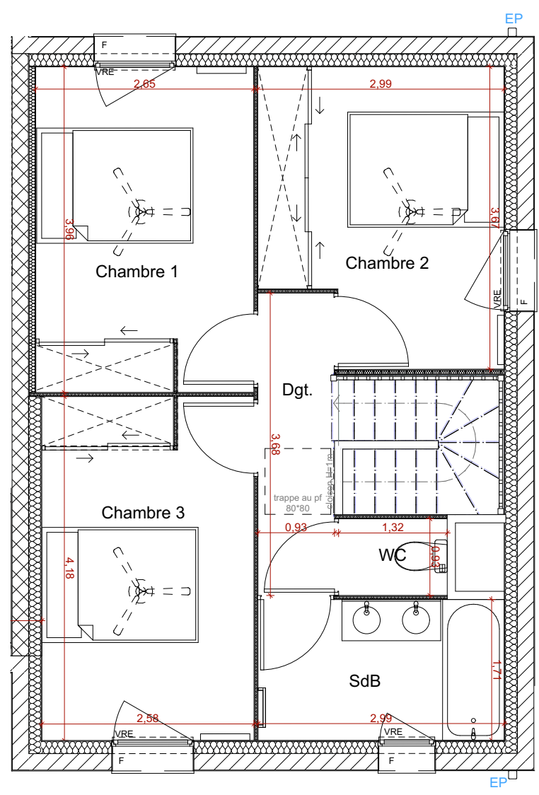
PLAN R+1
