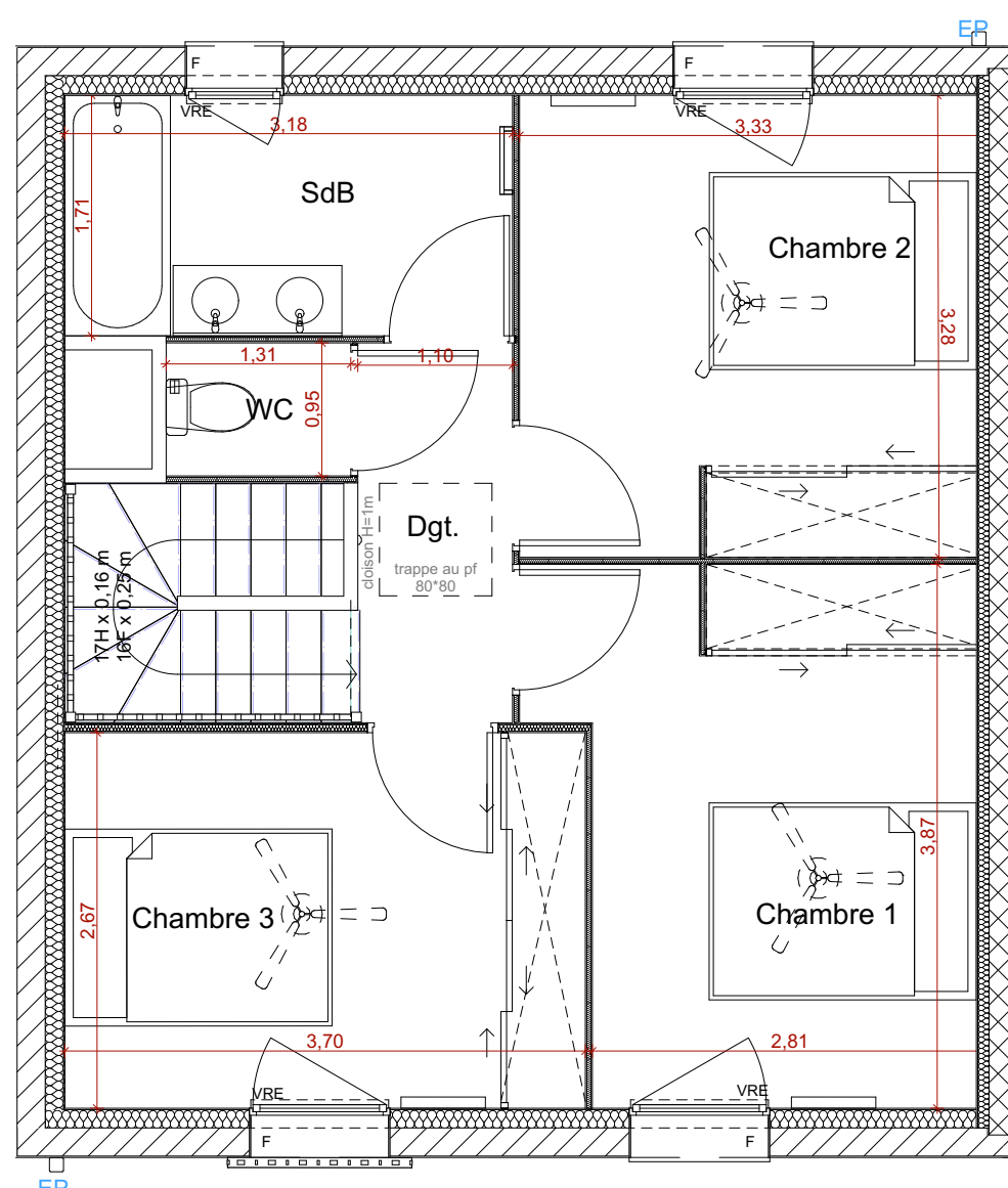
PLAN R+1
