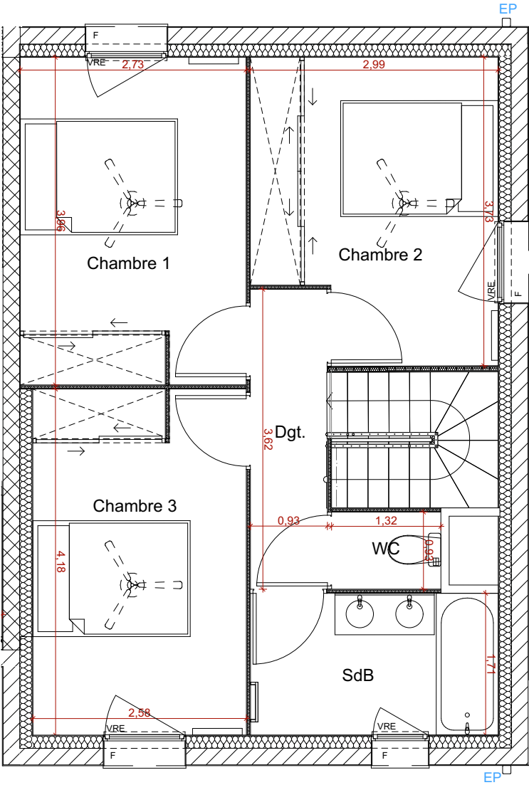
PLAN R+1
