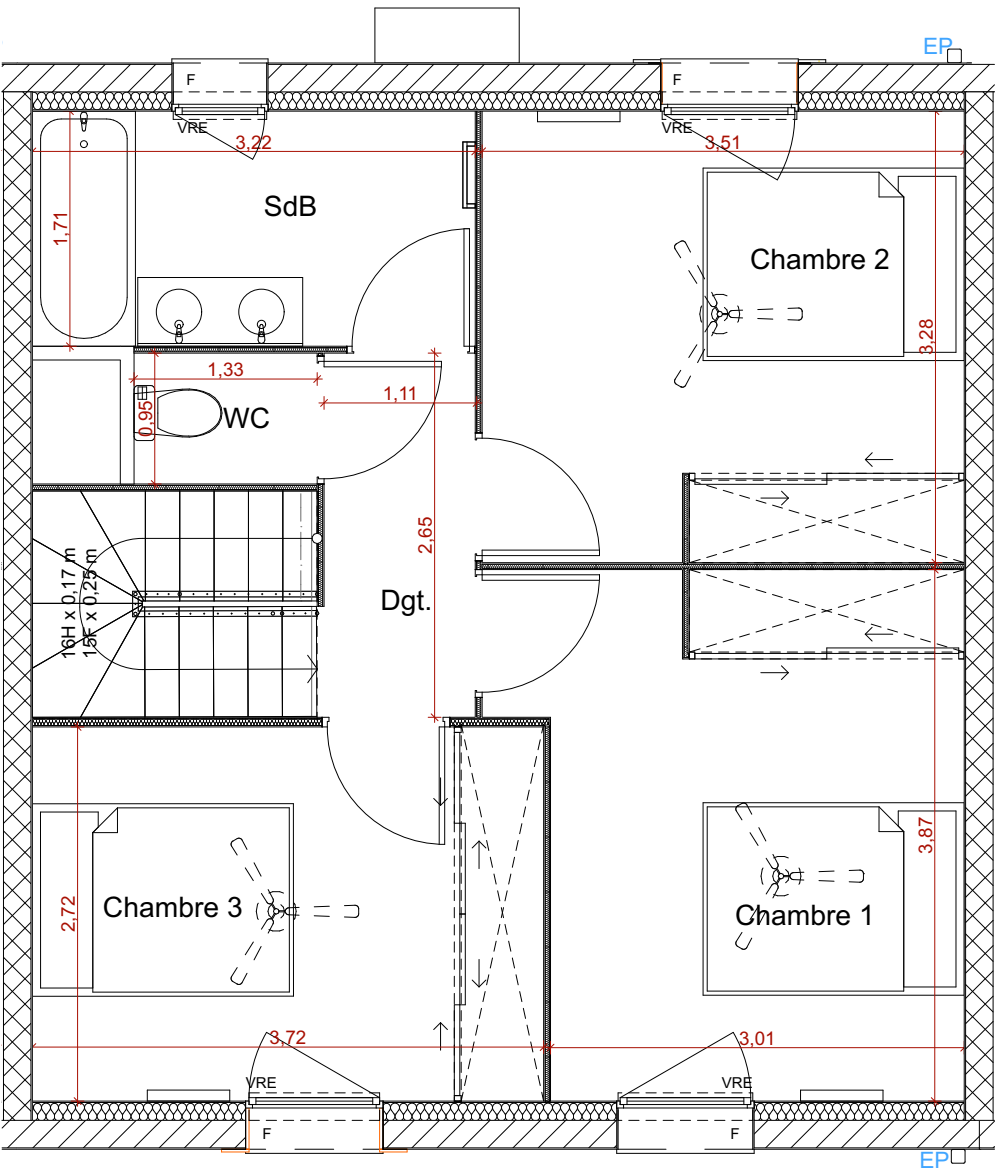
PLAN R+1
